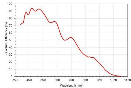
MER2-507-23GM NIR
